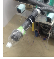
Fig. 4. Manipulator's end-effector with sucking nozzle of cleaner.
