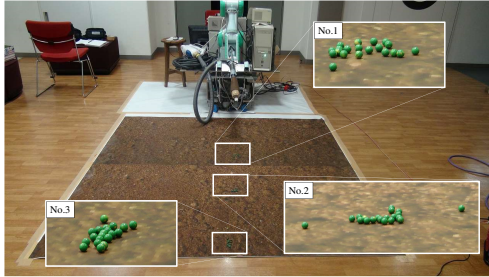
Fig. 5. Experiment Condition for 3D Recognition of Green particles placed on soil-photographed-clothes with three groups of particles.
