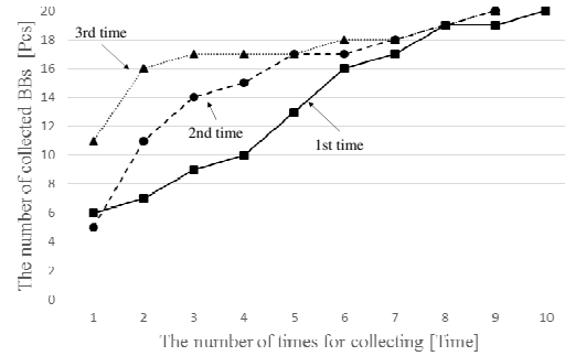
Fig. 8. Relationship between the number of sucked particles and the number of sucking trials. The total number of the particles is twenty, having certified the sucking all particles is successfully completed.
