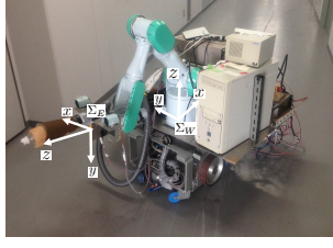
Fig. 3. Mobile manipulator with a sucking head, and vehicle coordinates \Sigma_W fixed at the base link of mounted manipulator hand coordinates \Sigma_E .
