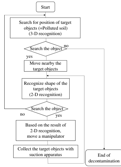
Fig. 2. Flowchart of autonomous behavior driven by environment conditions interpreted as instructions like programming, which can be thought to be environment programming.
