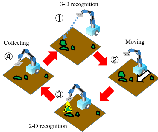
Fig. 1. Decontamination process composed of (1) finding 3D position of GPs, (2) approaching there, (3) reconfirming the 2D position when the hand-eye camera of the mobile manipulator looking down the GPs from just above the GPs' position, (4) sucking the GPs by cleaner.
